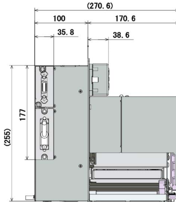
Figure 7-4b, Interface Side
